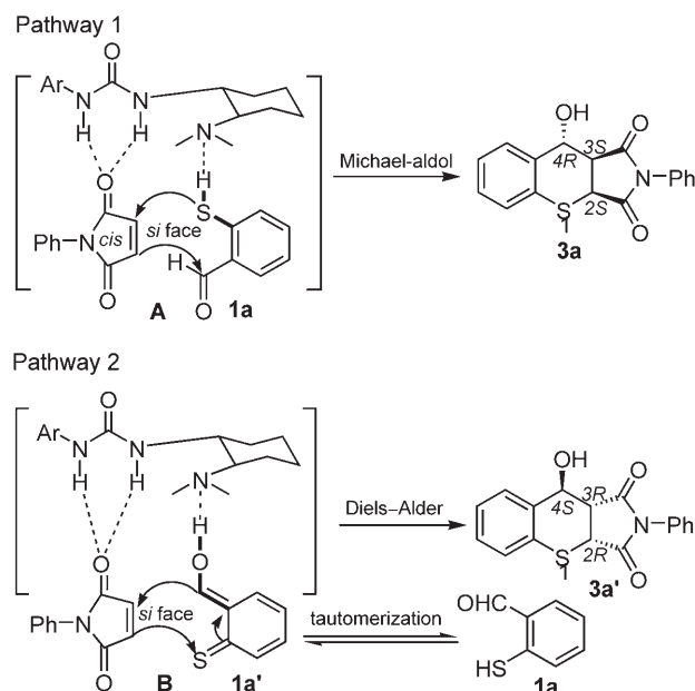
Figure 3. Proposed transition states.
