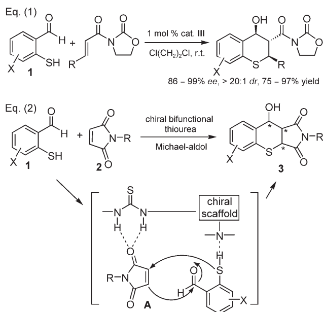
Scheme 1. Organocatalytic, asymmetric domino Michael-aldol reactions.
