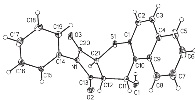
Figure 2. X-ray crystal structure of 3e .
